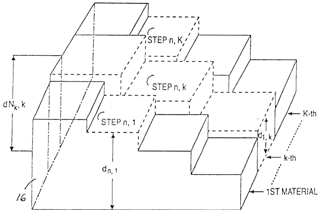
FIG. 4 PRIOR ART
